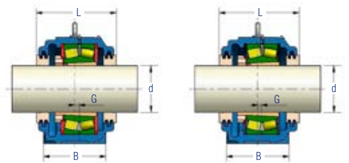
BP - Locating bearing, passing shaft
