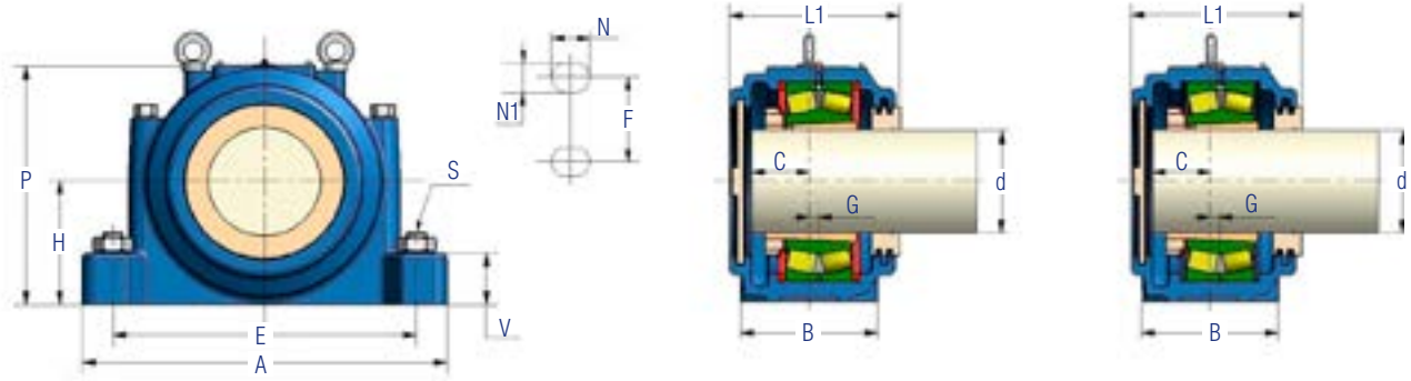
BC - Locating bearing, blind shaft
