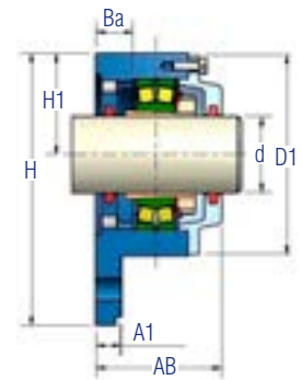
LP - Non-locating bearing, passing shaft
